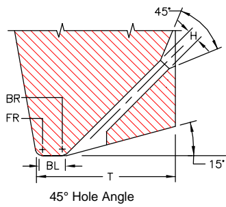
45° Hole Angle
